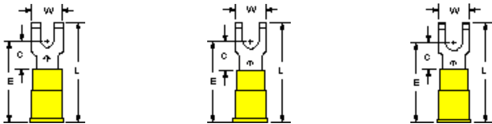
MVU10-6FFB MVU10-8FFB MVU10-10FFB Stud Size 6 8 10 Wire Range 12-10 12-10 12-10
